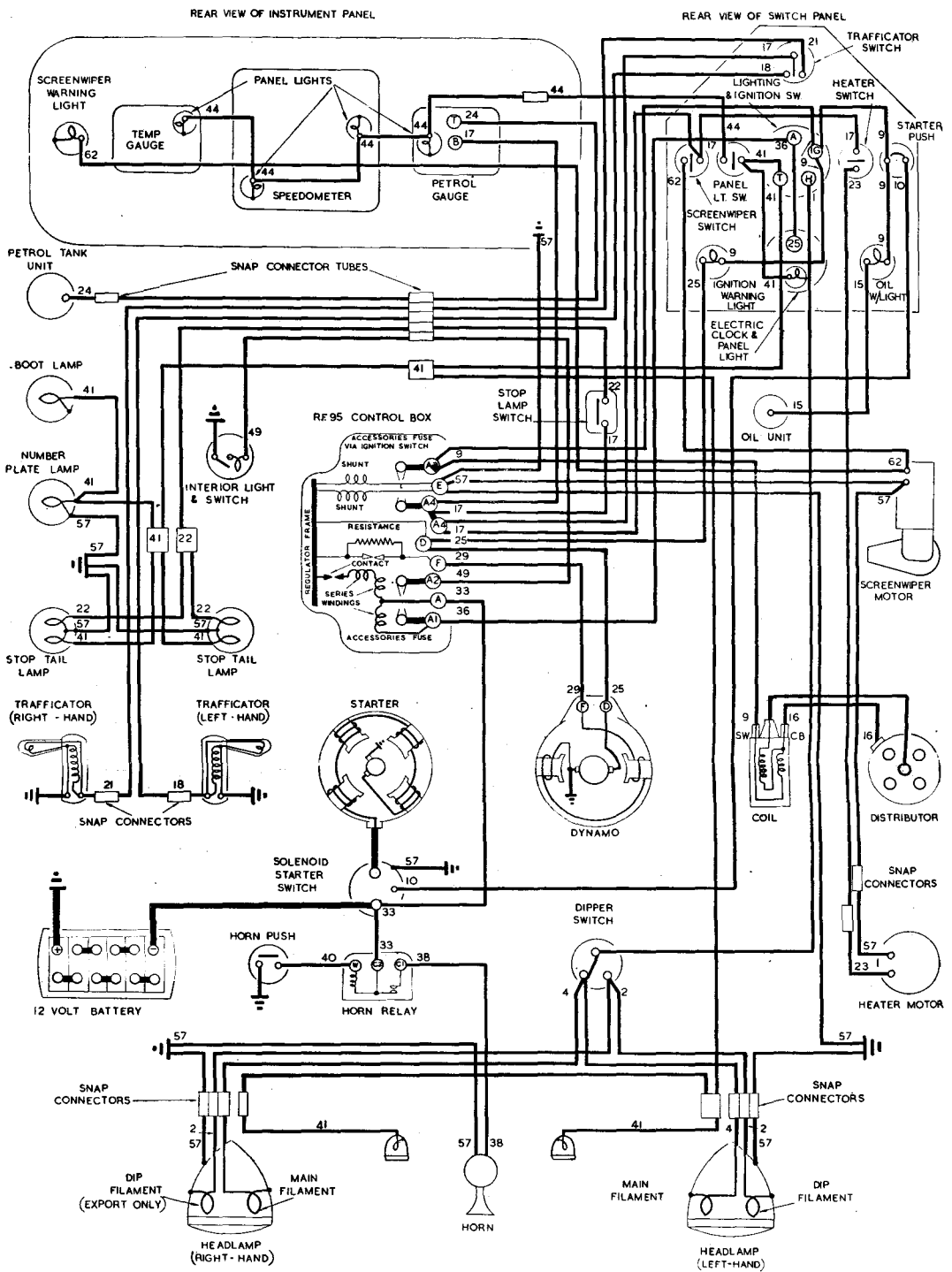
JAVELIN STANDARD SALOON R.H.D.—Figure 32 WIRING DIAGRAM, KEY TO CABLE COLOURS.
